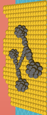
Nanocar 3–4 nanometres
